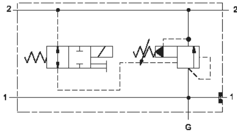
Normally Open
